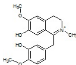
1,2-Dehydroreticuline
